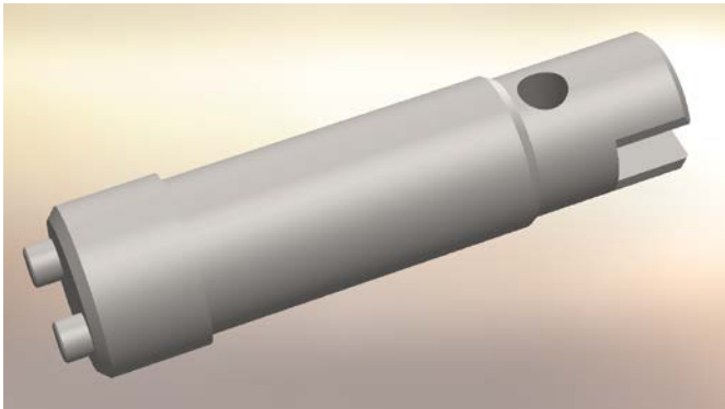
600.0104 Support shank – Longblade – (P125)
