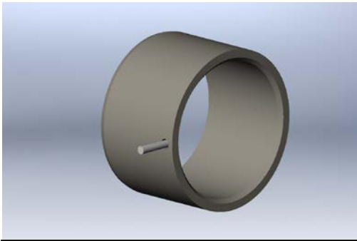
600.0203 Slide bushing – P180 1010-0028 Conical Pin 3x16
